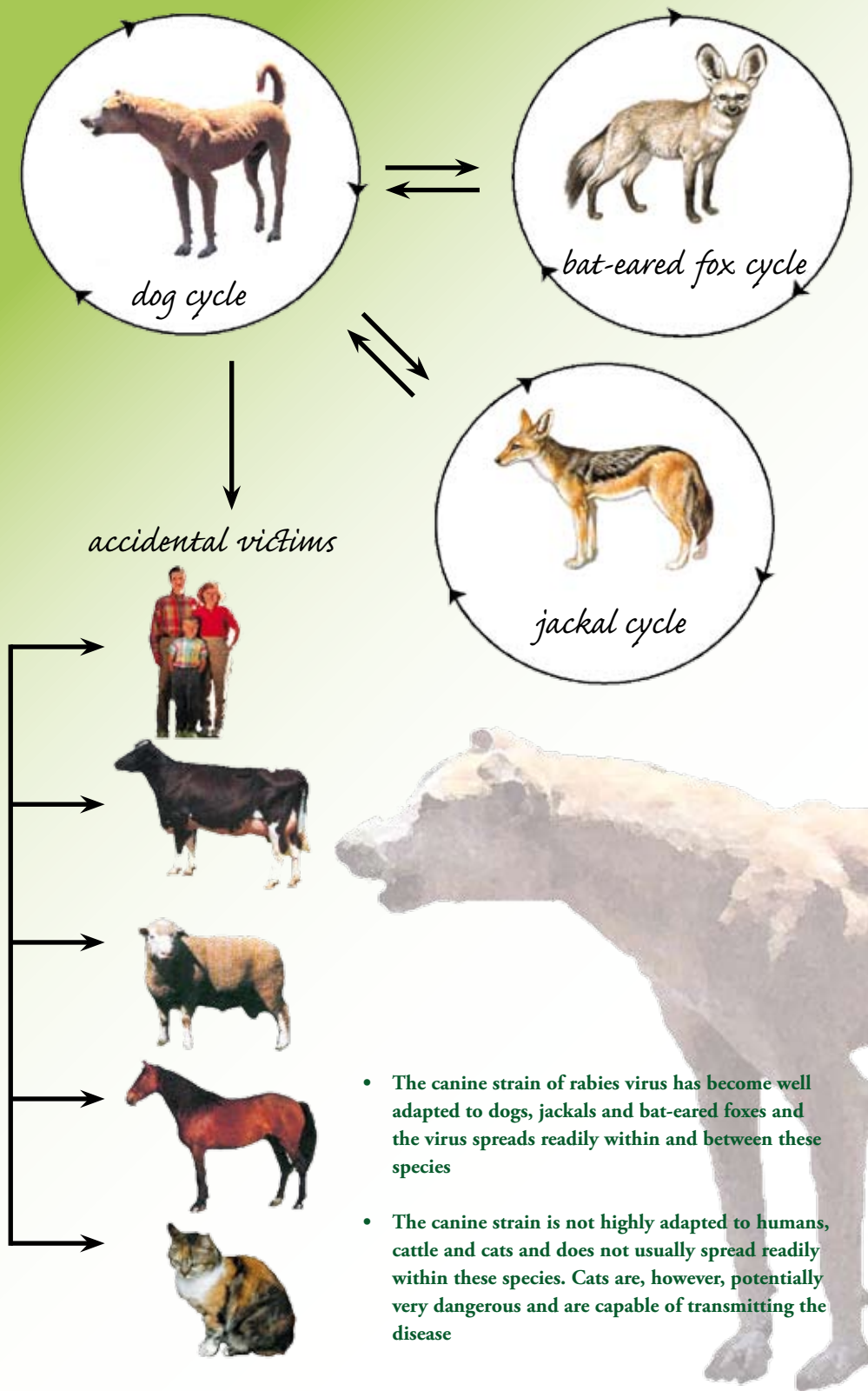
Fig.1: An illustration of canid rabies virus strain cycles in various species
