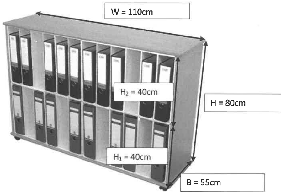
Figure 9: Movable Laboratory Lever Arch Files Storage Unit
