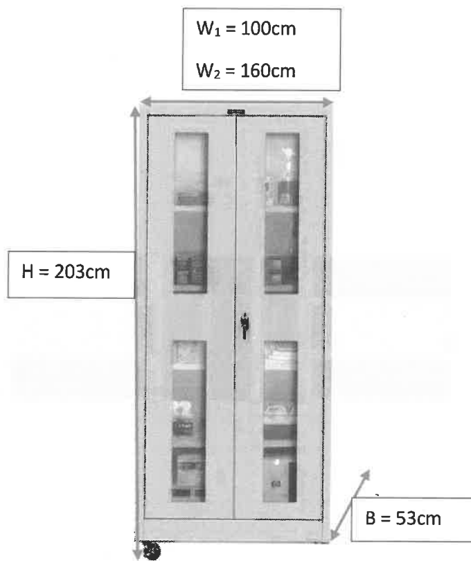
Figure 16: Storage Cabinet on Wheels with see-through doors
