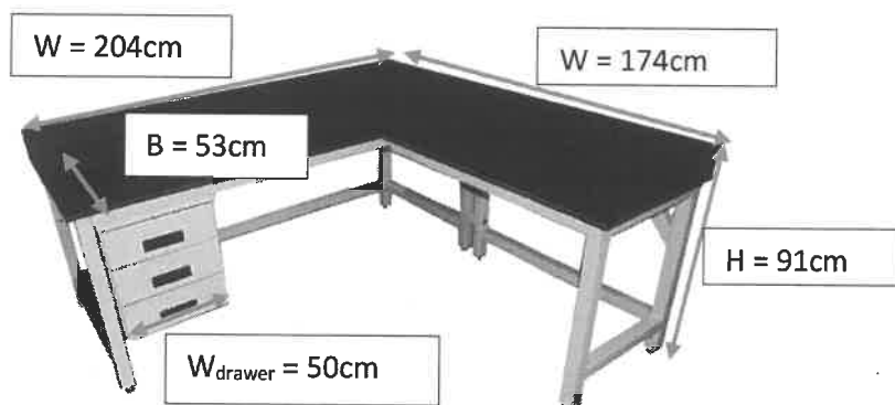
Figure 15: L-shaped workbench with drawers and cabinet with double doors
