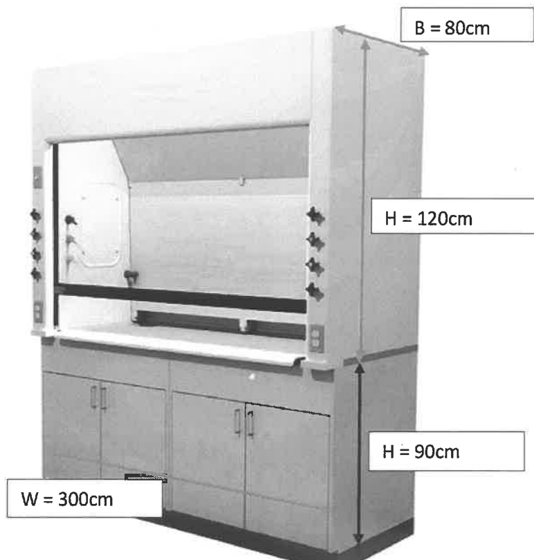
Figure 2: Laboratory Fume hood with storage cabinet
