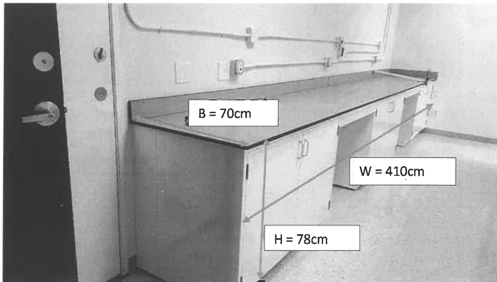
Figure 1: Laboratory Workbench with Double Doors
