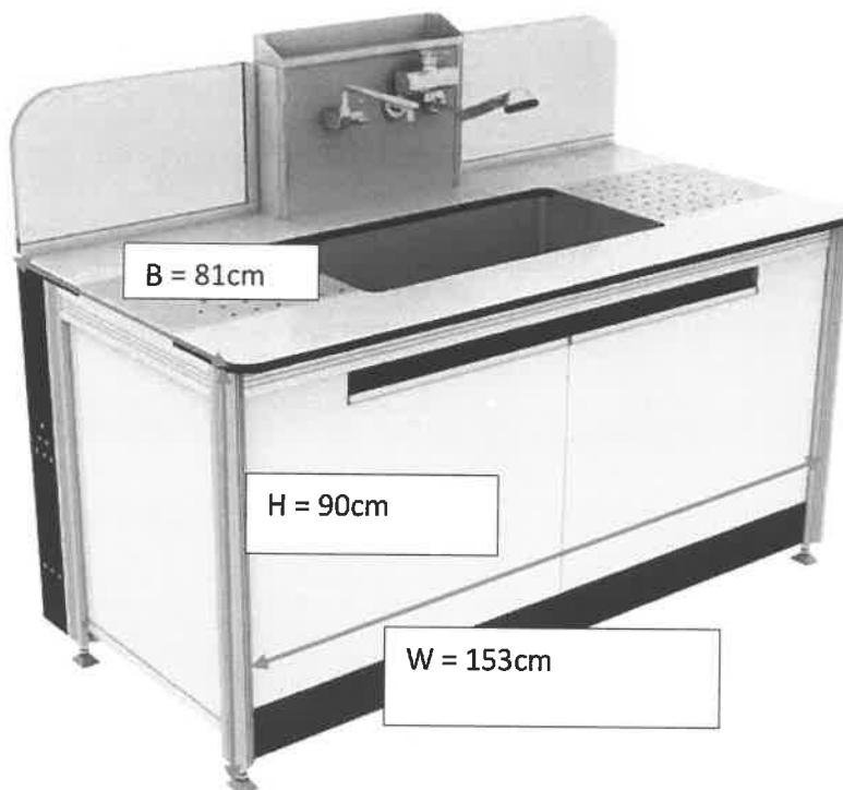
Figure 8: Laboratory Stainless Steel Sink Table with Doors
