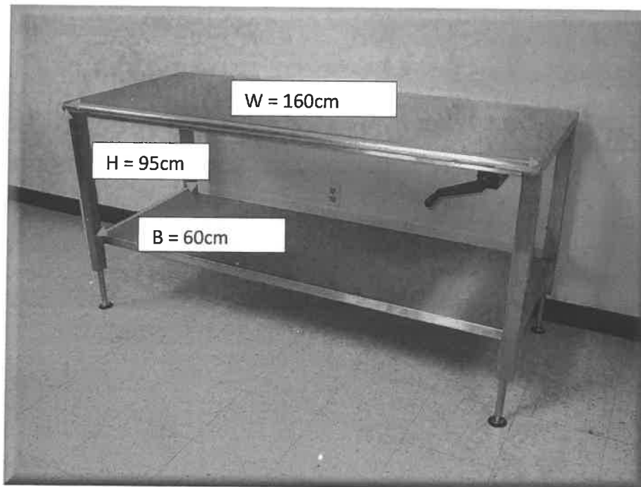
Figure 7: Laboratory Stainless Steel Workbench
